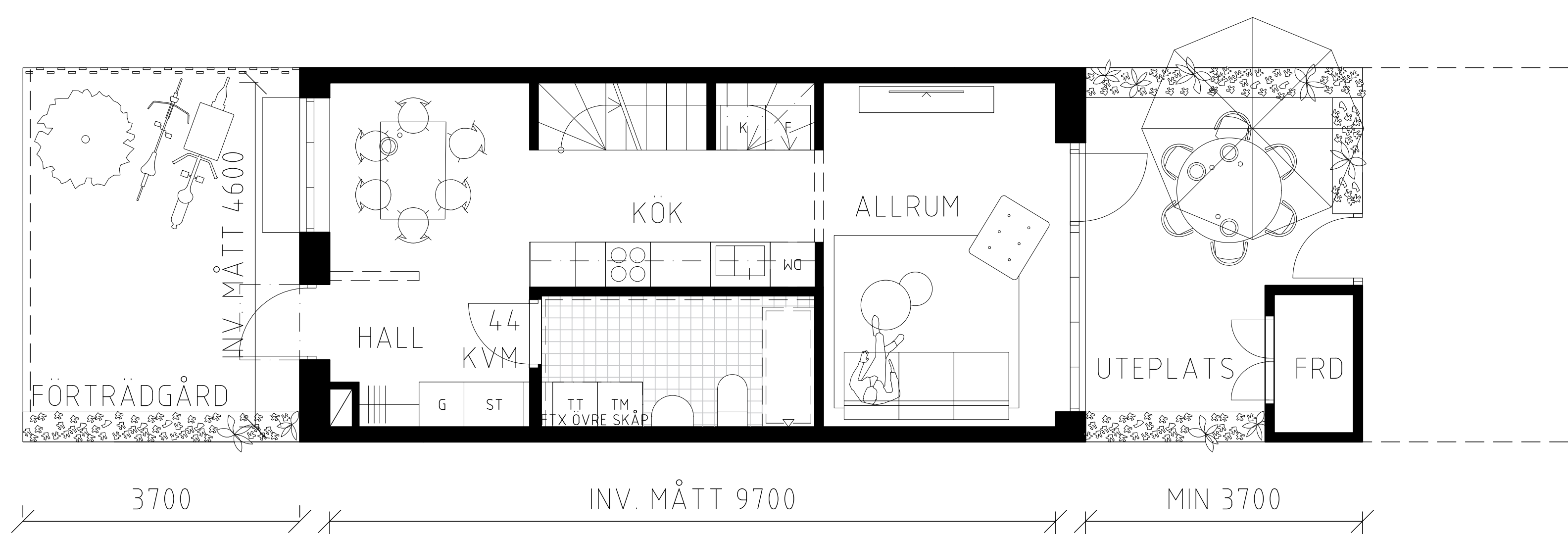
Plan Radhus 4rok 1:50
